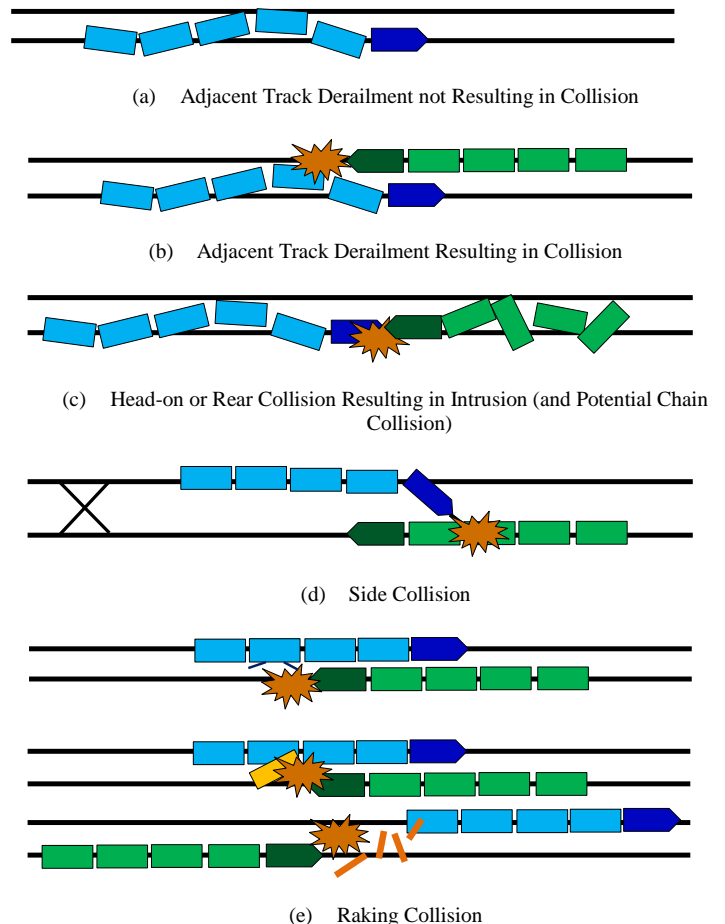
Fig. 4. Specific ATA Derailment and Collision Scenarios
